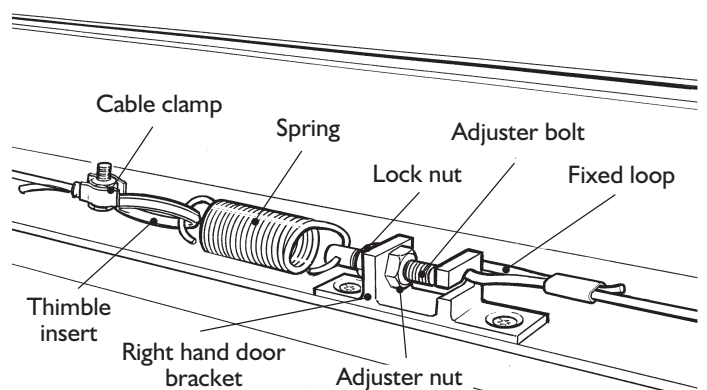
Diagram 4. Cable anchored to right hand door, tensioning and adjustment bolt.
