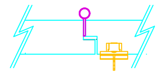
VIEW E: EXAMPLE REBATED DOOR
